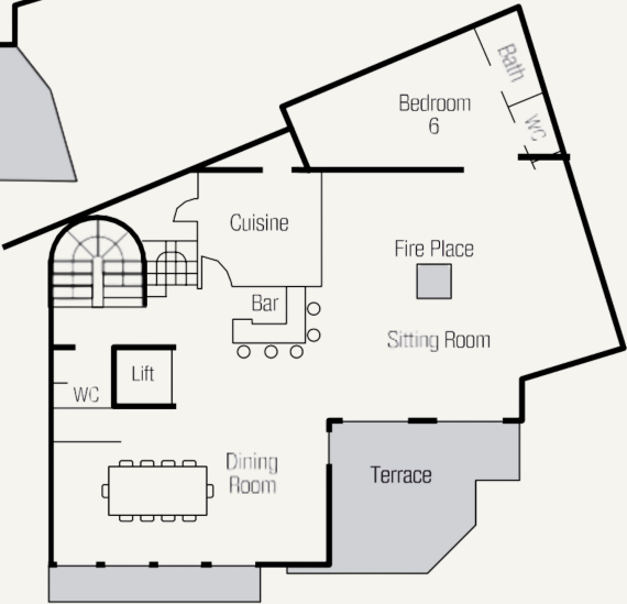
LEVEL 2
